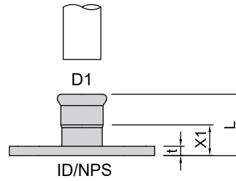
Dimension 't' includes any raised face height unless otherwise noted.
