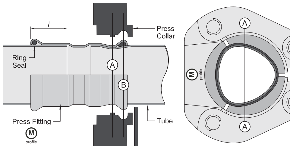
Above: Lemon shape section profile - Before pressing (fitting left), after pressing (fitting right) & Section A through pressed joint.
