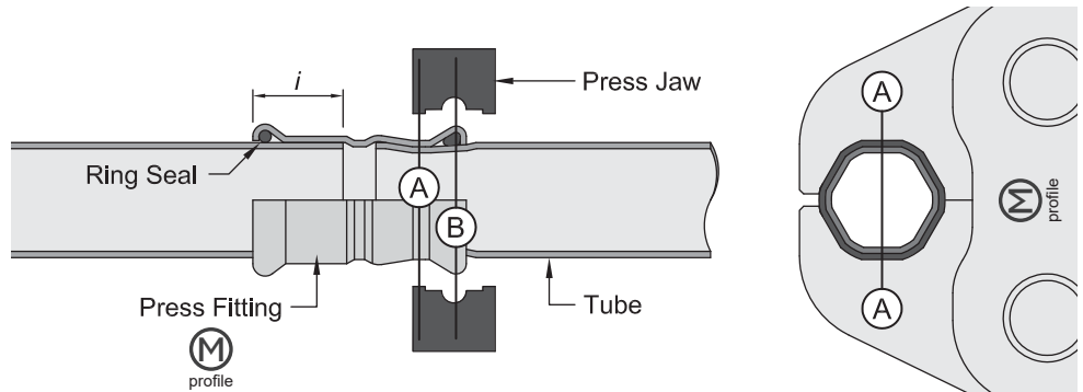
Above: Press Tools are fitted with an interchangeable jaw or, adaptor jaw and collar combination depending on the fitting material, system diameter and fitting press profile to be pressed. All must match for the press to be successful.
