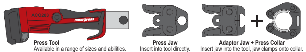
Above: Press Tools are fitted with an interchangeable jaw or, adaptor jaw and collar combination depending on the fitting material, system diameter and fitting press profile to be pressed. All must match for the press to be successful.
